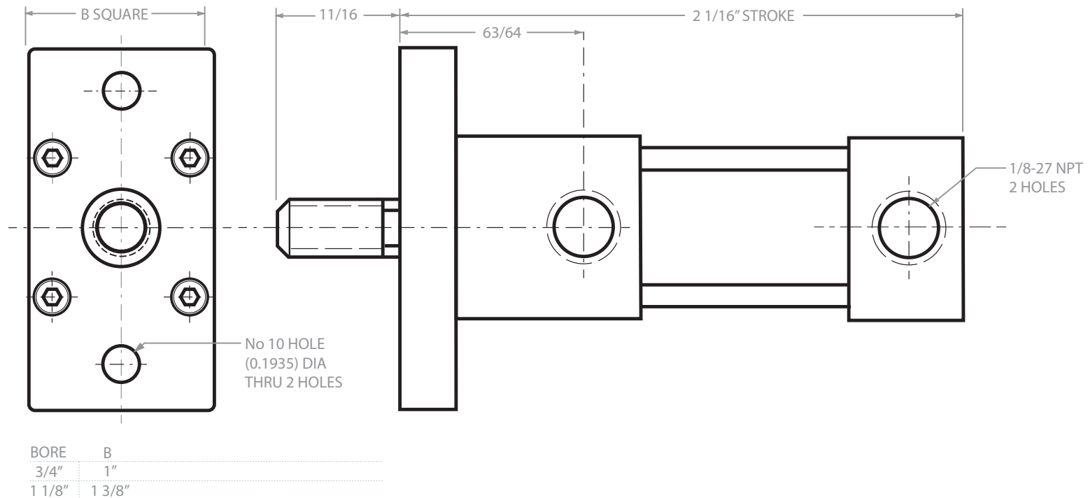
LITTLE AIR GIANT AIR CYLINDER • MODEL LG-REF • REAR END FLANGE
